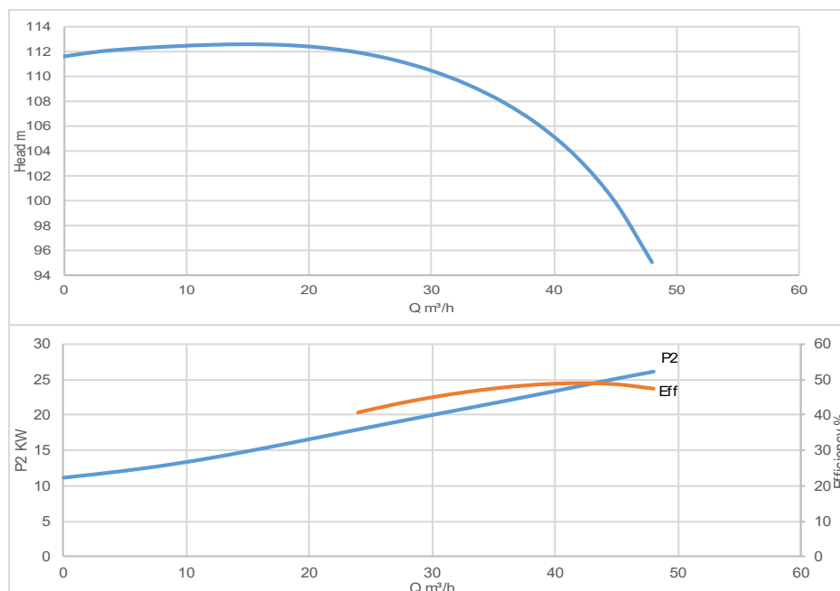
Performance Curve
