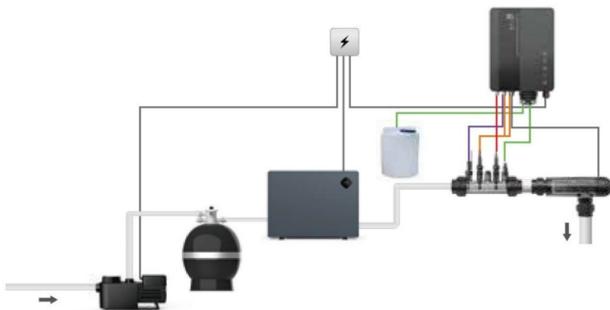
① Installationsdiagram
