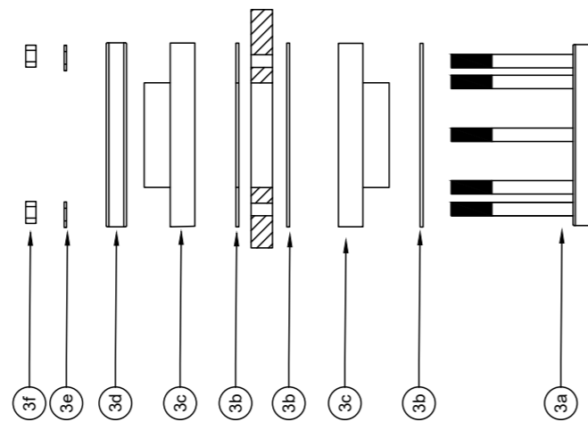
Filter wall
