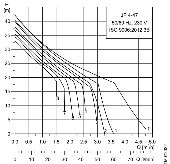
JP 4-47 performance curves for suction lifts of 0 to 8 m
