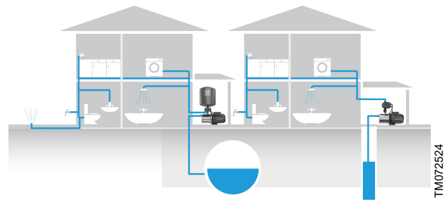
Examples of applications with JP Boosters
