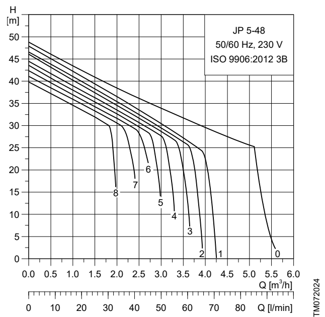
JP 5-48 performance curves for suction lifts of 0 to 8 m
