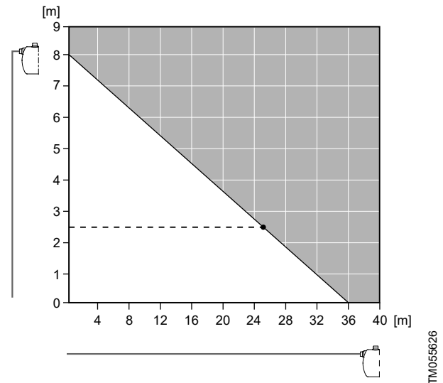
Maximum inlet-pipe length (horizontal axis) according to the suction lift (vertical axis)
