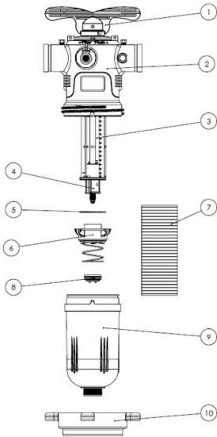
Exploded View
