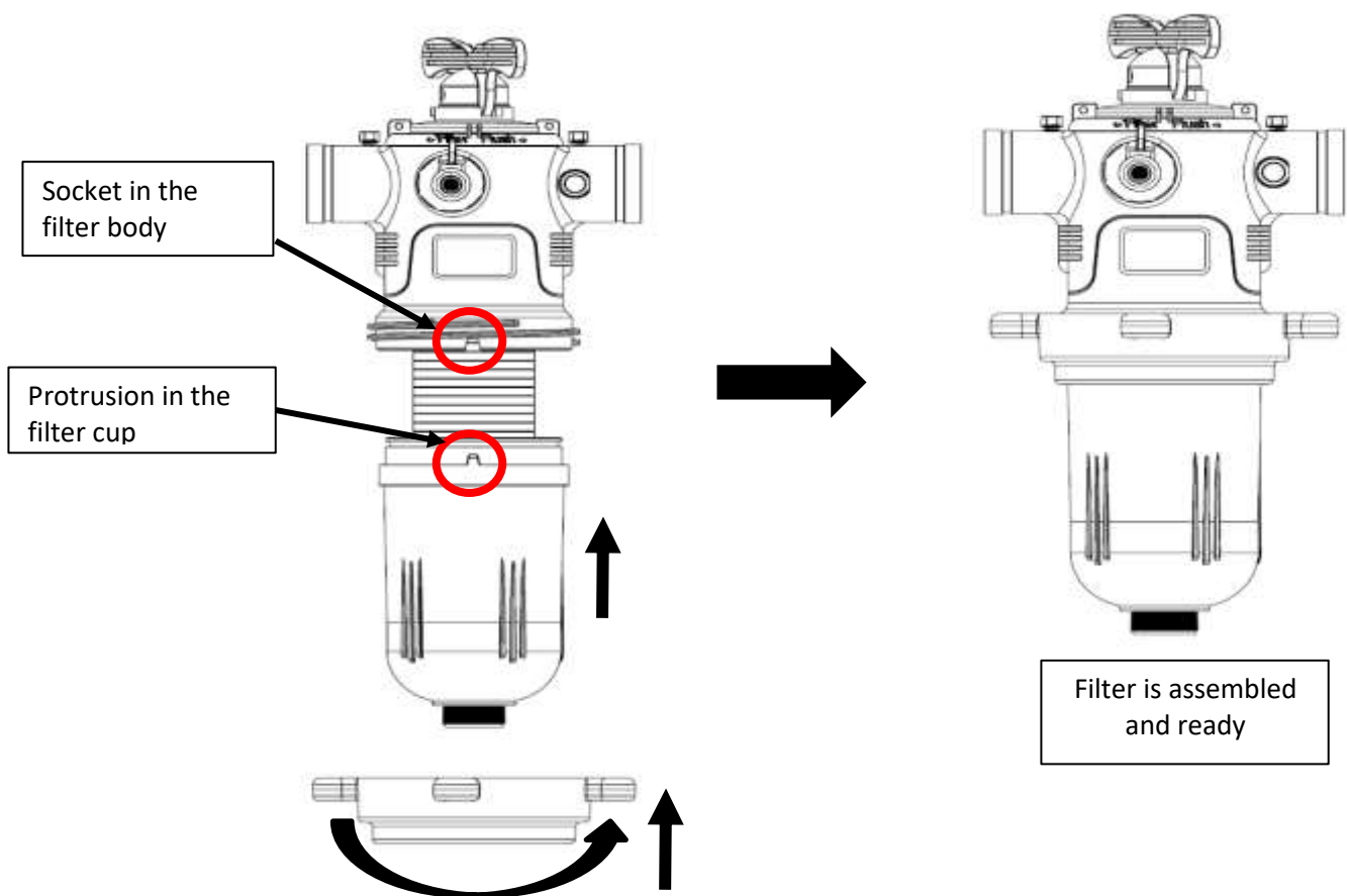
Cup assembly and tightening the locking ring
