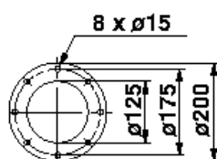
Pump with Grundfos flange
