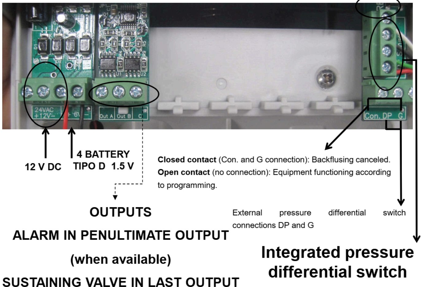
AZUD FBC 209T 12 V DC CONTROLLER GRAPHIC CHART
