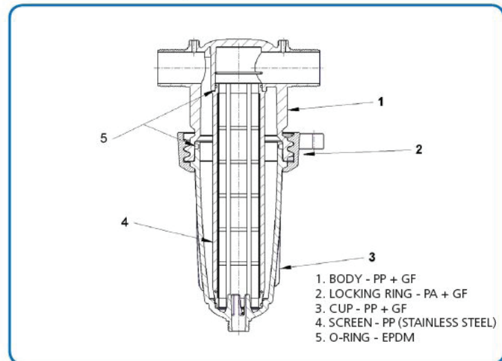
1", 1 1/2" SCREEN FILTER
