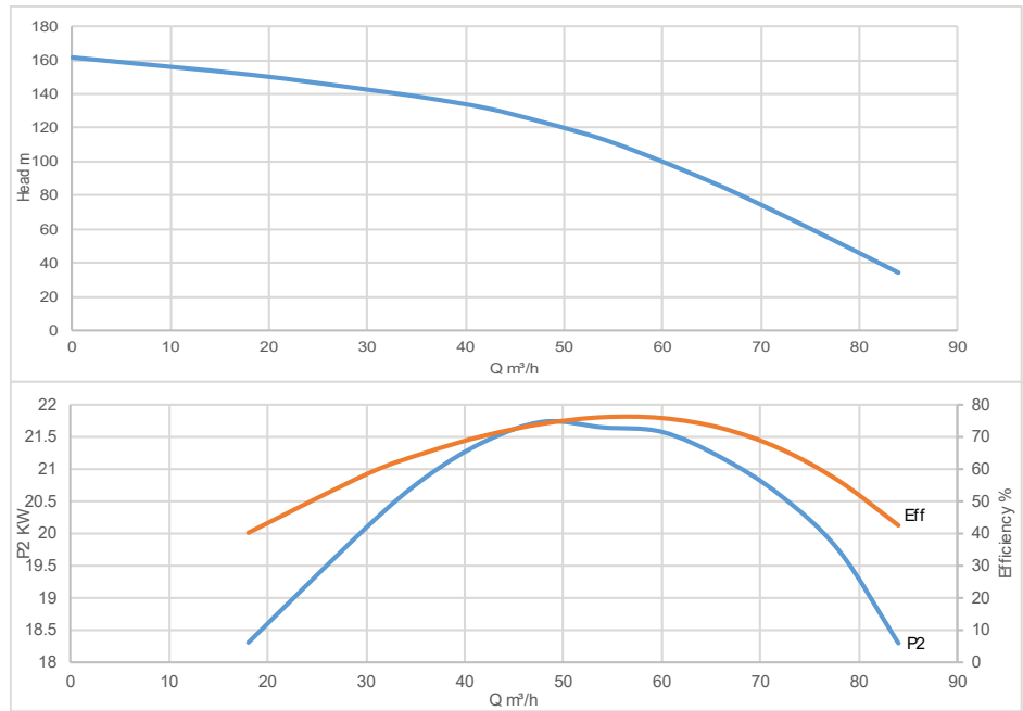
Performance Curve
