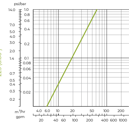
Head Loss Graph (in clean water)
