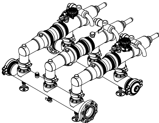
3 units of 4" Mini Sigma for flow rates up to 240 m³/h (1,057 gpm)
