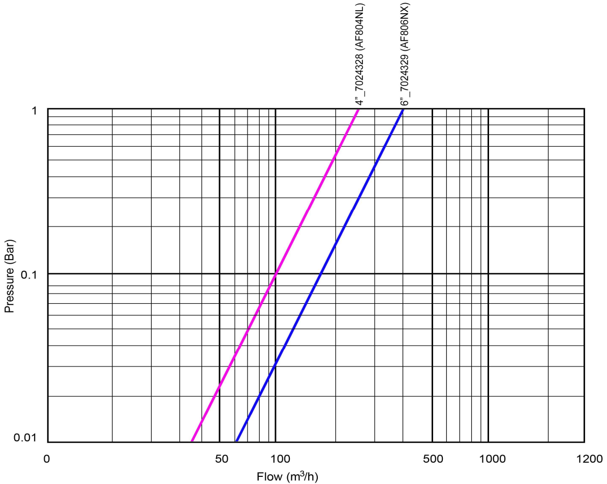
GRAPH-Pressure loss at 120 micron
