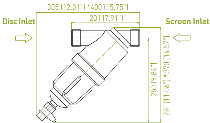
Dimentional Drawing
