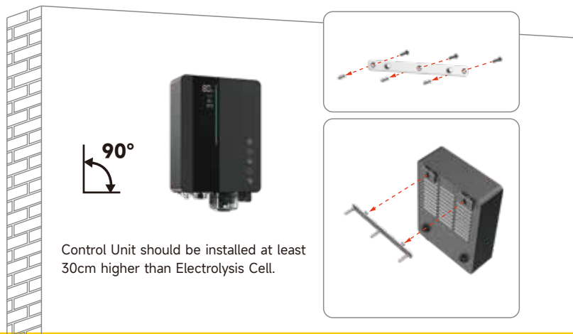
③ Control Unit Installation
